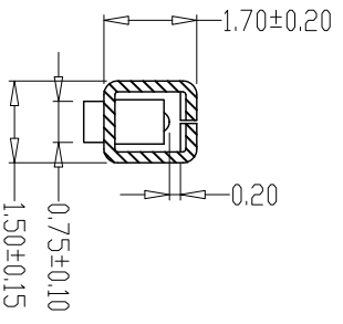
SEC:C-C
